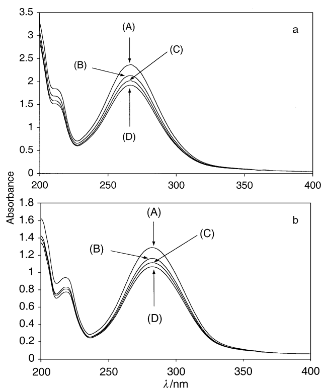
Fig. 1 Spectra of (a) 1.62 \times 10^{-4} M nitrobenzene and (b) 1.46 \times 10^{-4} M 4-nitrotoluene aq. 1% SDS solutions (5 ml) exposed to aligned carbon nanotubes (sample area ca. 1 cm 2 ) at 298 K. Spectra recorded after (A) 0, (B) 3, (C) 5 and (D) 7 days.
