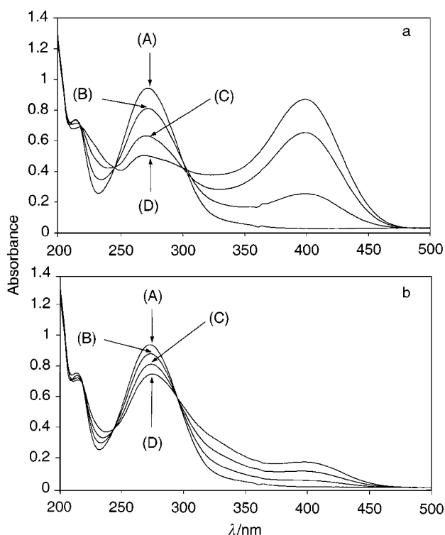
Fig. 2 UV-vis spectra showing hydrolysis of p NPA ( 5.0 \times 10^{-5} M) in an aq. 1% SDS solution (5 ml) at 298 K (a) with and (b) without exposure to aligned carbon nanotubes (sample area ca. 1 cm 2 ) at 298 K. Spectra recorded after (A) 0, (B) 7, (C) 14 and (D) 21 days.
